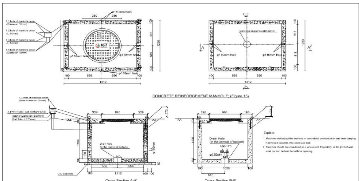
Figure 3-14 Manhole Design
