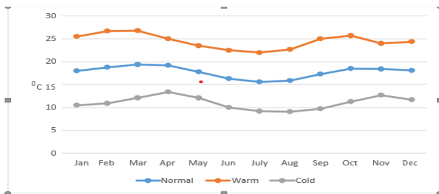
Graph 1: Average temperature per month
