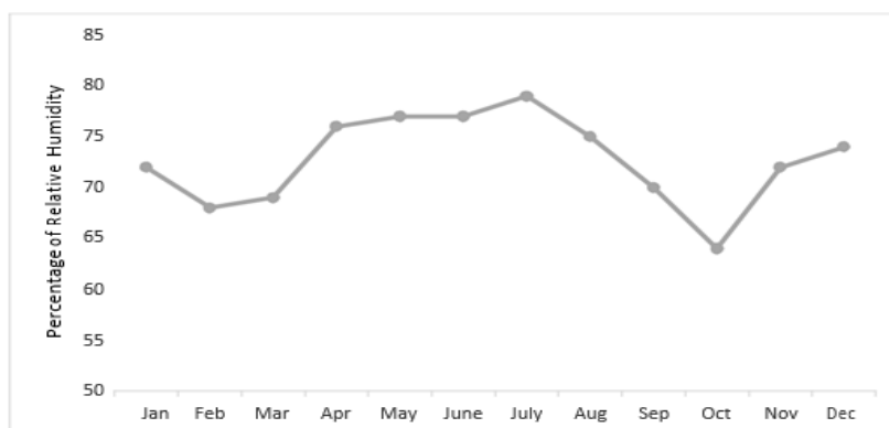
Graph 2: Mean relative humidity percentage
