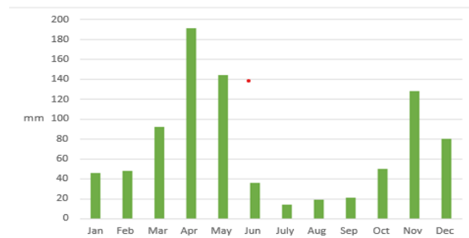
Graph 3: Precipitation rate in mm
